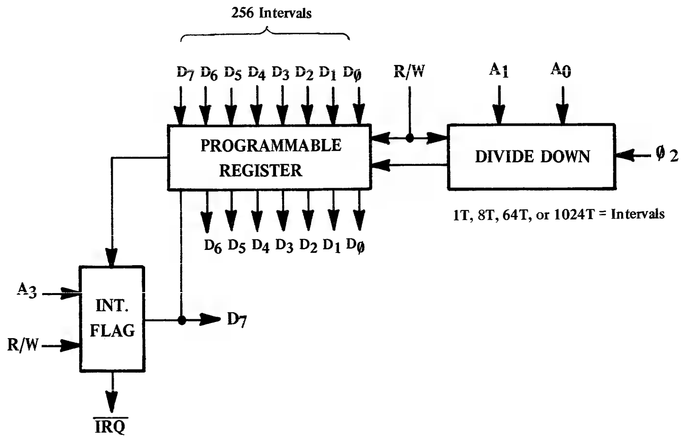
Basic Elements of Interval Timer
